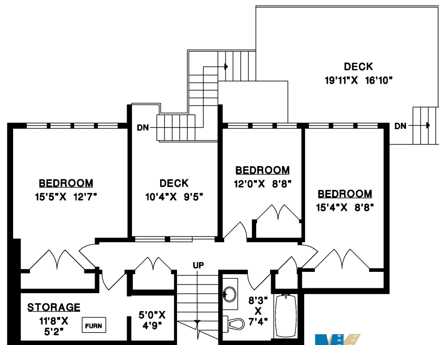
BOTTOM FLOOR
