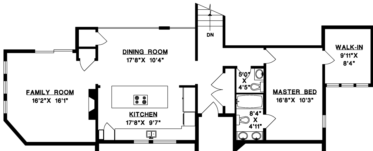
MAIN FLOOR
